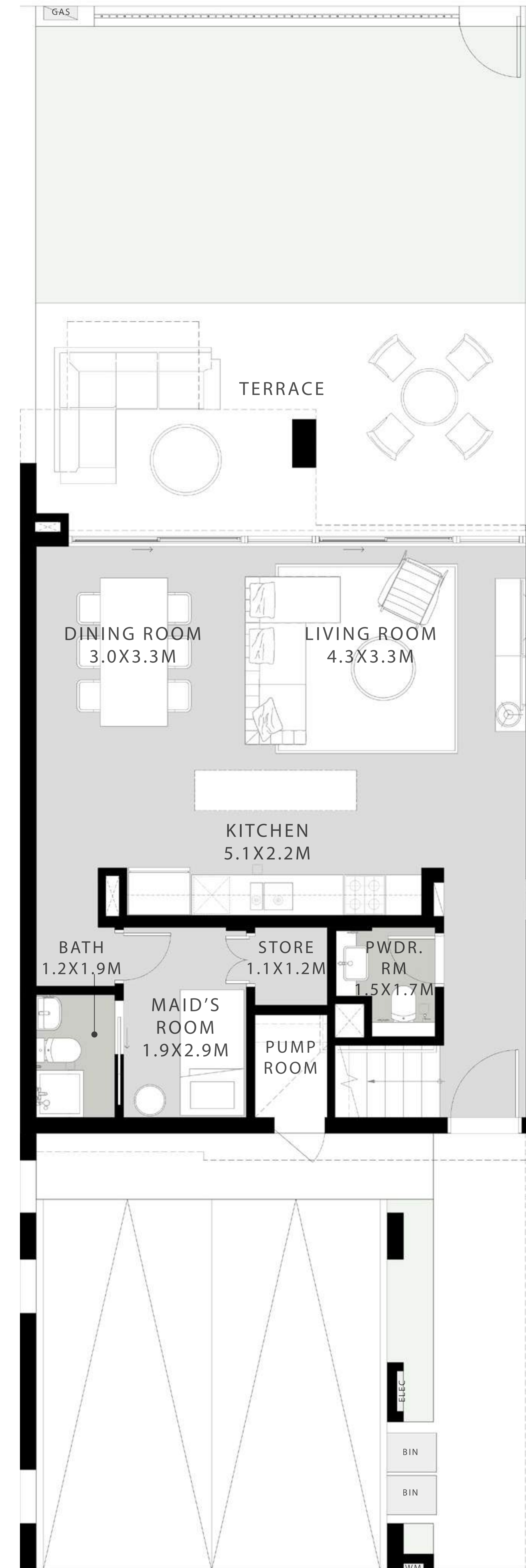
GROUND FLOOR
