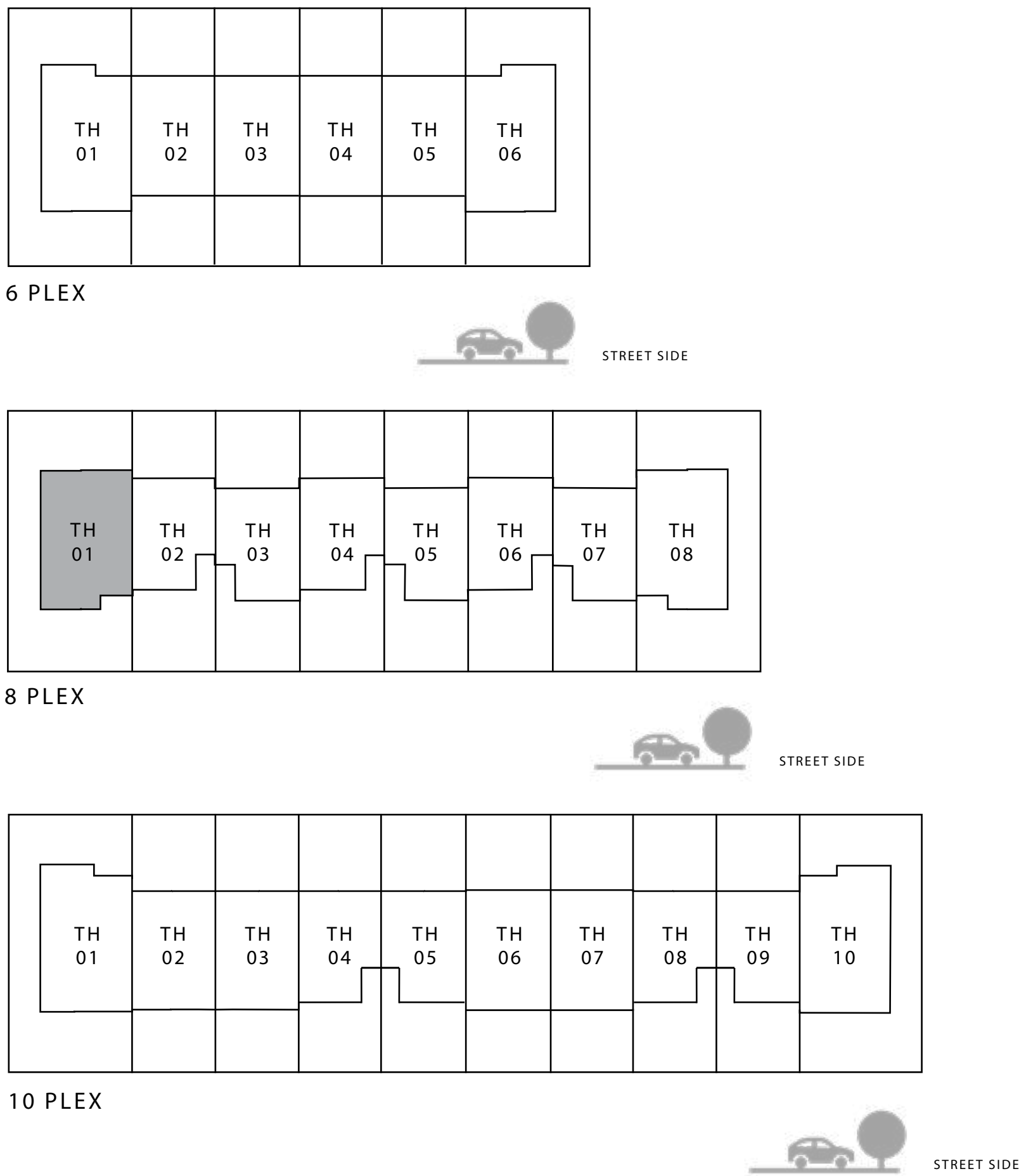
KEY PLAN
