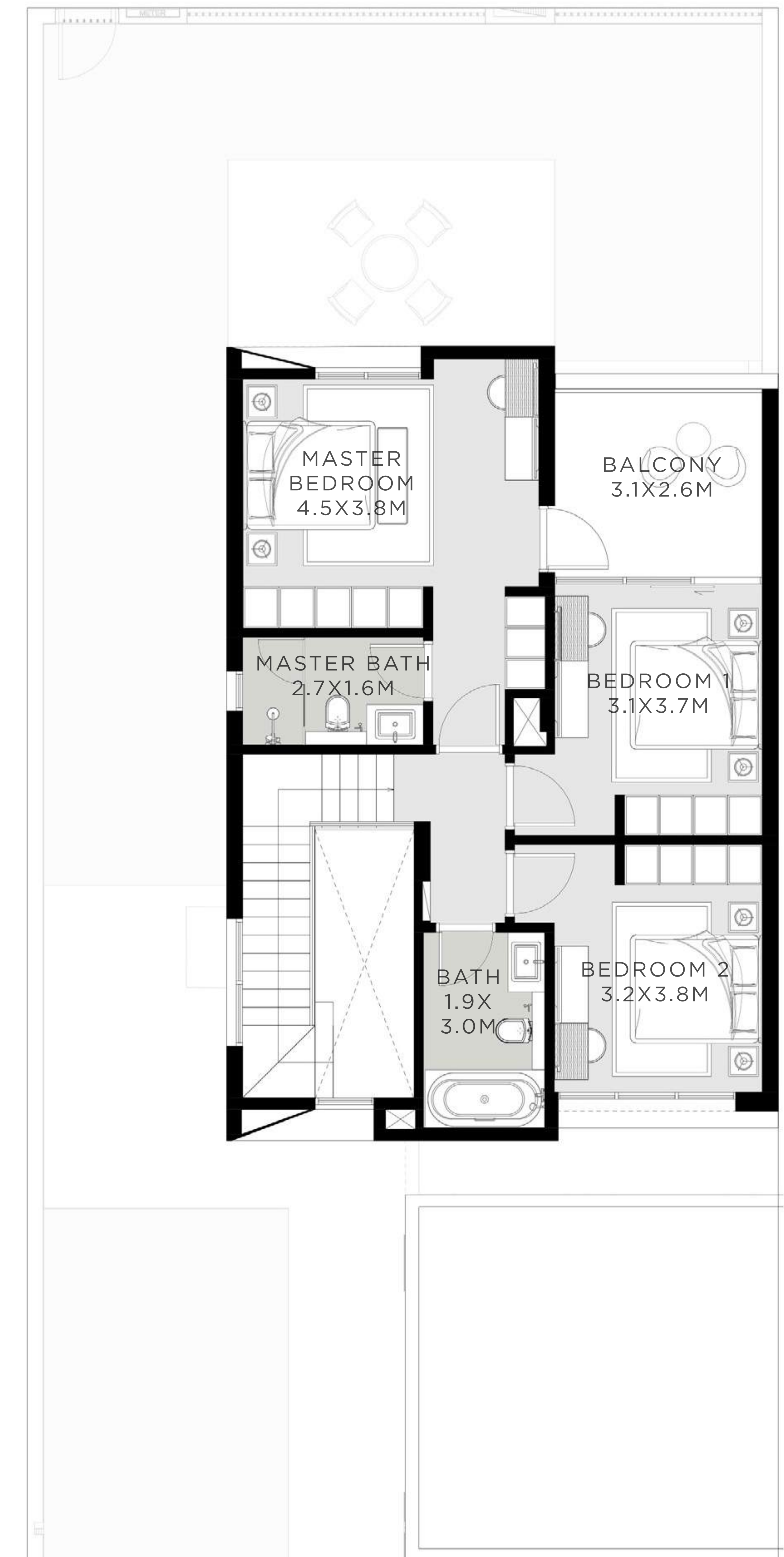
FIRST FLOOR
