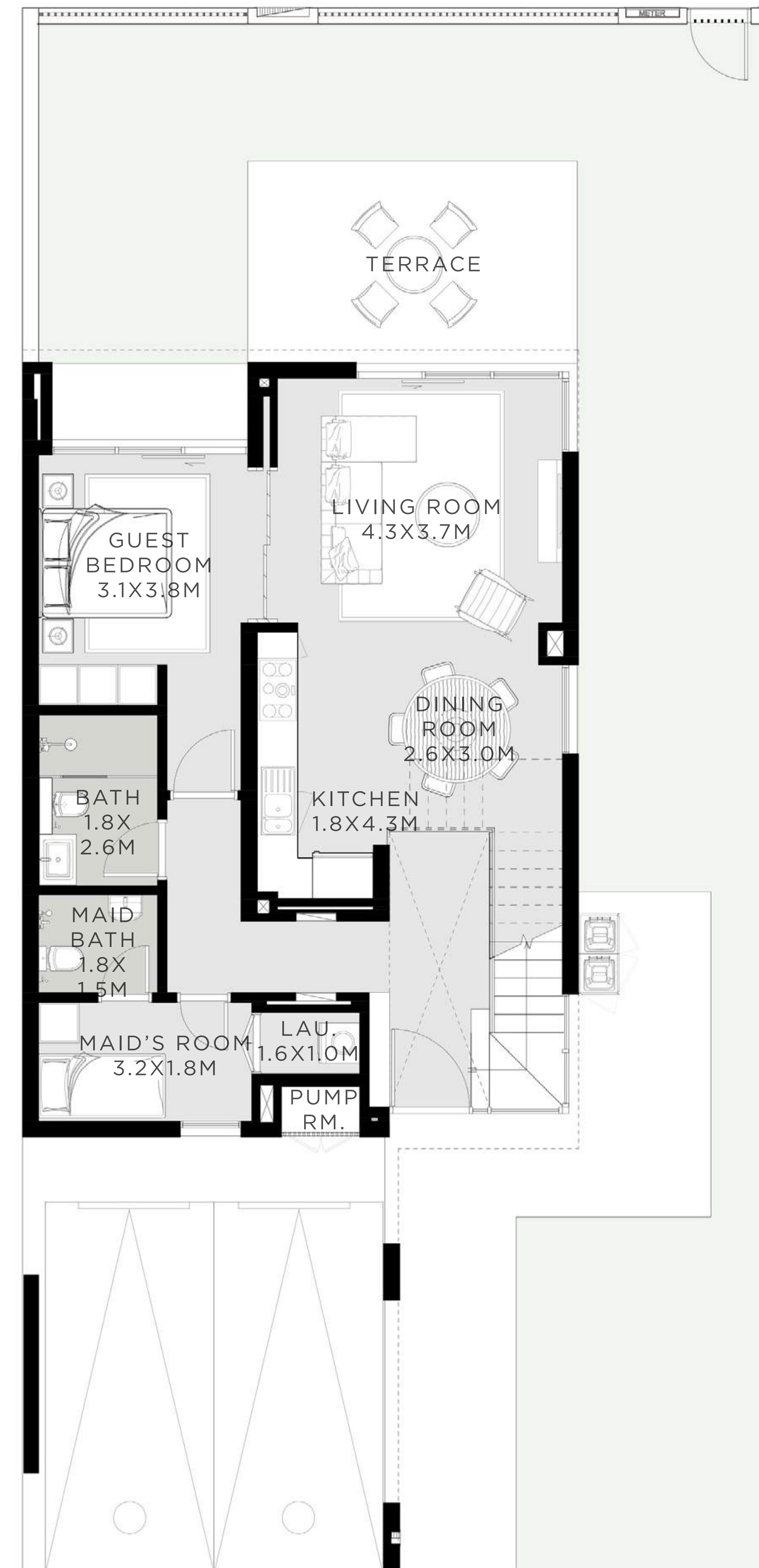
GROUND FLOOR
