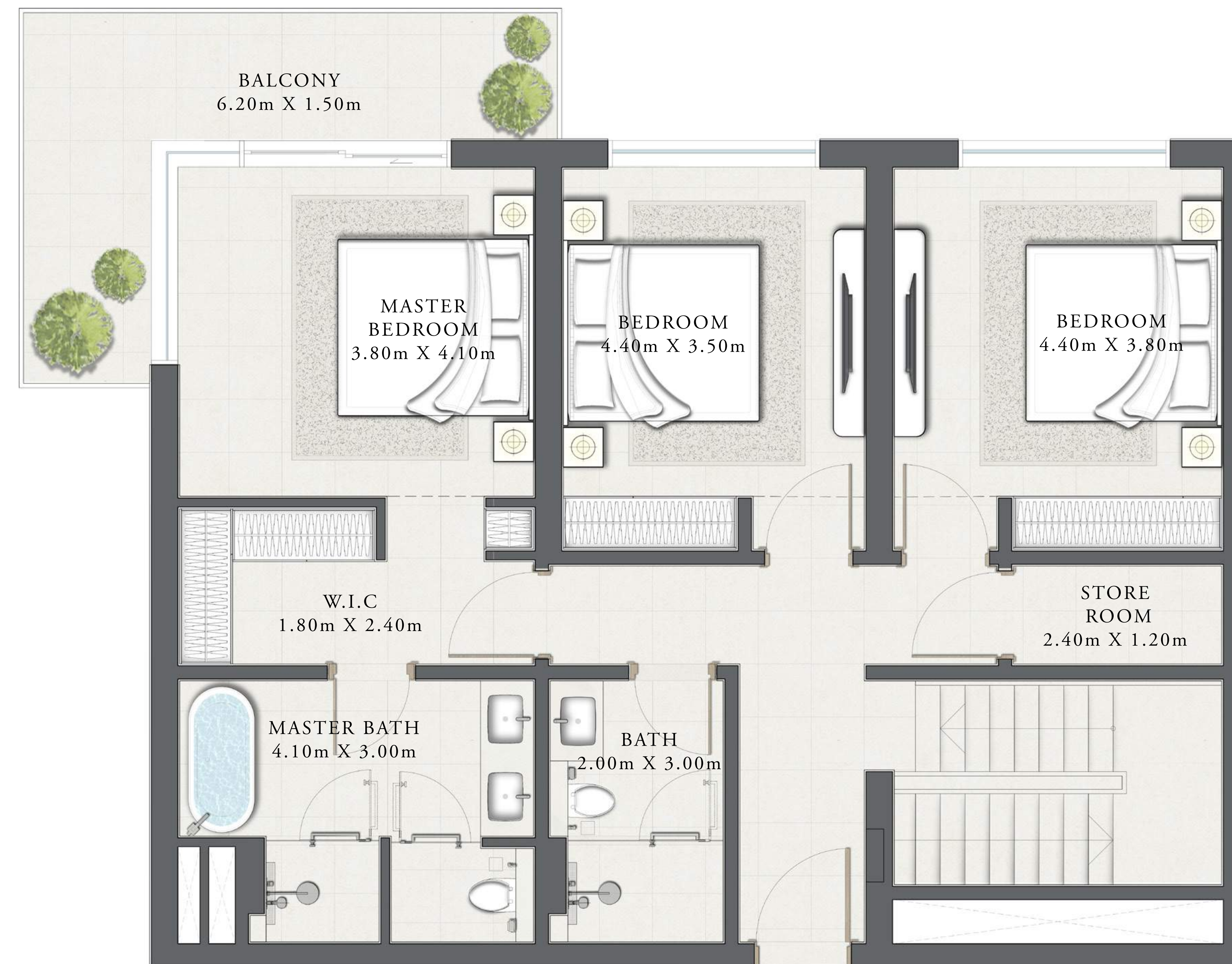
UPPER LEVEL
