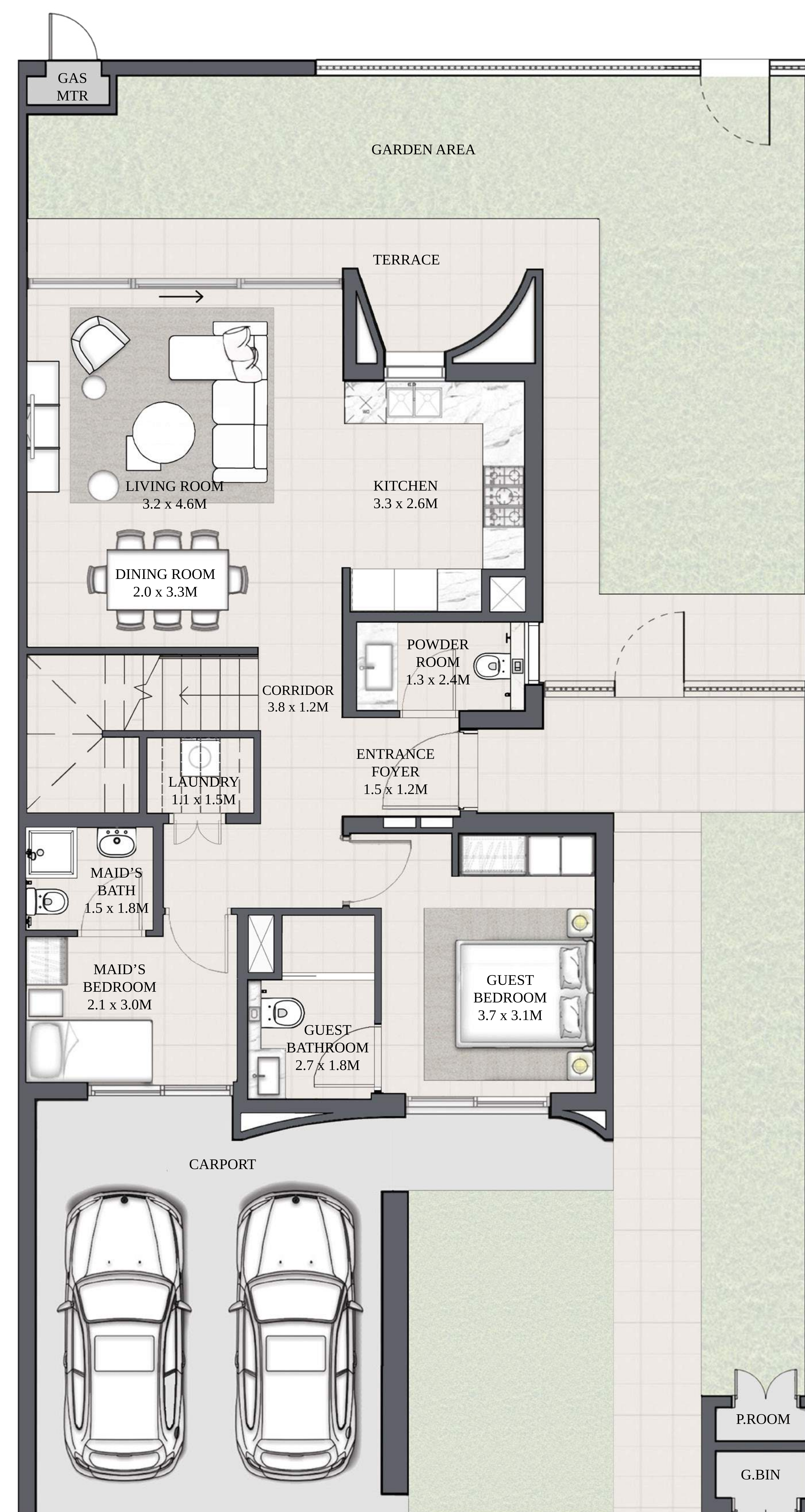
GROUND FLOOR
