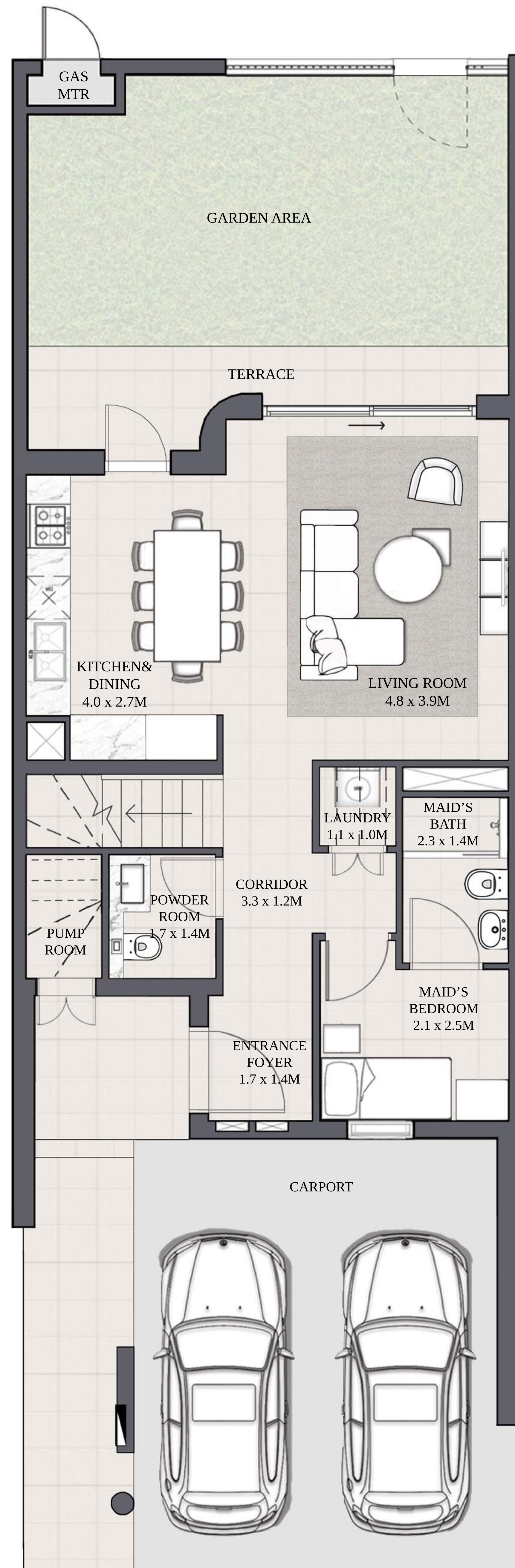
GROUND FLOOR
