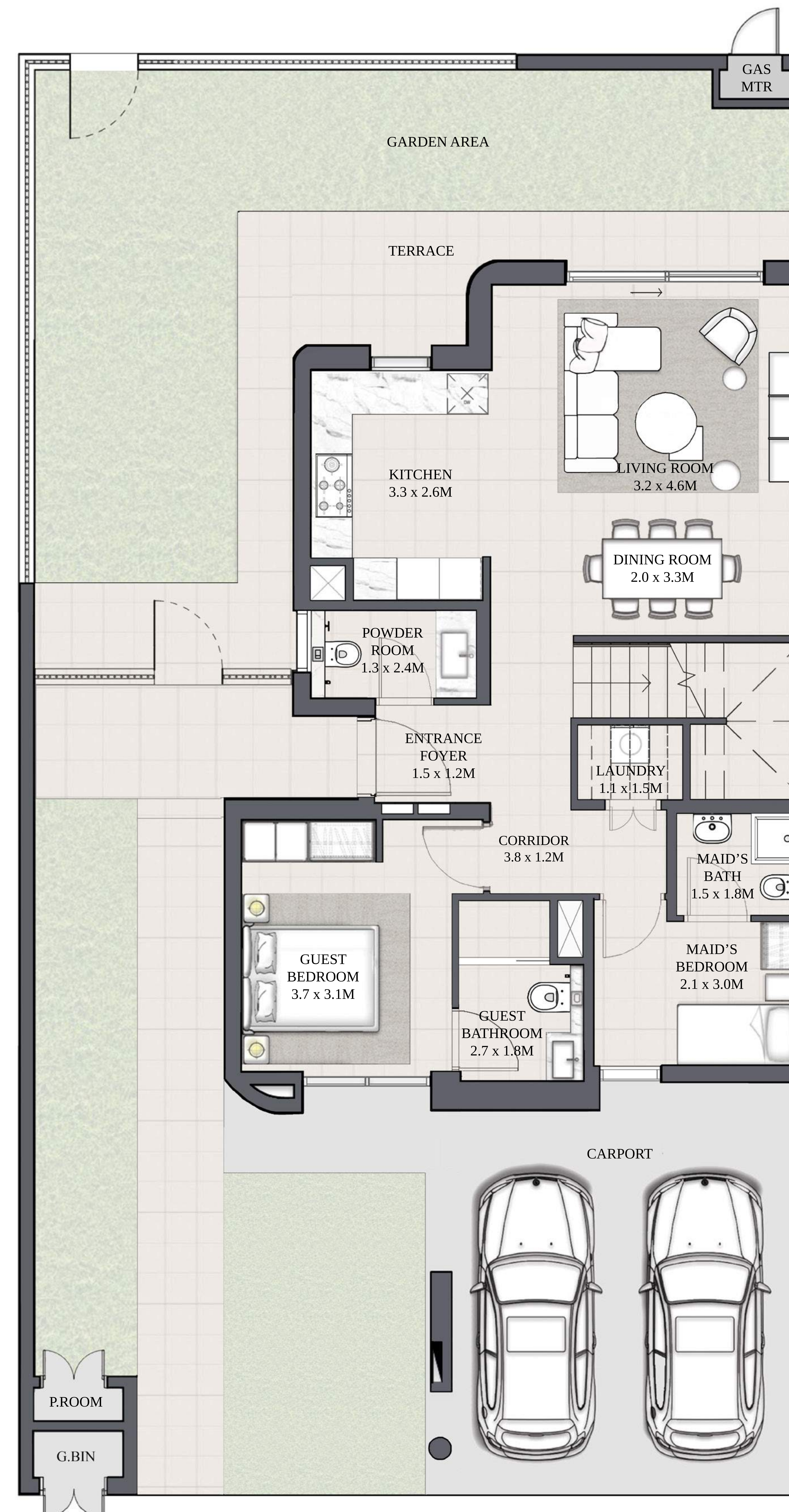
GROUND FLOOR
